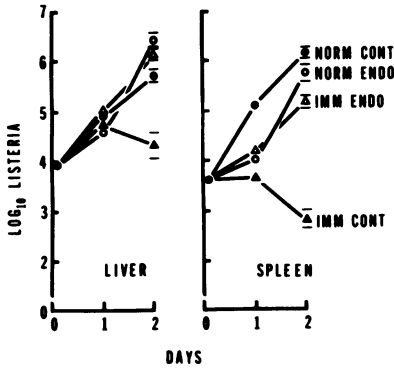
FIG. 2. Suppression of expression of adoptive immunization by the injection of 25 \mu g of endotoxin into recipient mice 4 h before the infusion of immune cells and an intravenous Listeria challenge of 10^5 cells (IMM ENDO). Endotoxin greatly suppressed the protective effect of immune spleen cells (IMM CONT) and resulted in bacterial growth comparable to that measured in the livers and spleens of normal controls (NORM CONT) and endotoxin-treated controls (NORM ENDO). Means of five mice per time point \pm 2 standard errors.
