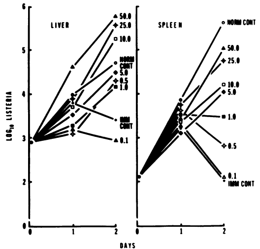
FIG. 3. Dose dependence of suppressive effect of endotoxin on expression of adoptive immunity. Shown are the suppressive effects on the expression of adoptive immunity of doses ranging from 0.1 to 50 \mu g given to recipient mice 4 h before the infusion of immune spleen cells and a Listeria challenge of 10^5 cells. As little as 0.5 \mu g caused significant suppression of adoptive immunity, and the suppressive effect increased with increasing dosage. Means of five mice per time point.
