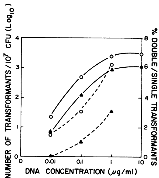
FIG. 3. Frequency of transformation of B211 Bac - as a function of strain GS-5 Pfa + Str + DNA concentration. Symbols; ○—○, Pfa + ; ▲—▲, Str + ; ○—○, Pfa + Str + ; ▲—▲, Str + Bac + .
