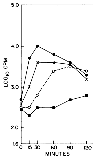
FIG. 5. Effect of catalase or DMSO on CL generated by the interaction of PMN, B. dermatitidis ( 10^6 ), and luminol ( 8 \mu g) in 10% fresh mouse serum. Shown are counts per minute produced by B. dermatitidis plus activated PMN alone (●), with 300 mM DMSO (×), or with 20,000 U of catalase per ml (■). Also shown are counts per minute generated by elicited PMN plus B. dermatitidis (○) under the same conditions.
