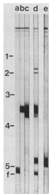
FIG. 1. Immunoblot of T. gondii cyst lysates probed with MAbs T8 3B1 (a), T8 4A12 (b), T8 2C2 (c), and T8 4G10 (e) and mouse serum taken prior to fusion (d). On this 12% acrylamide run, the 18-kDa antigen migrated with the front. The mobilities of standard proteins (Pharmacia LMW kit) were as follows: 1, 94 kDa; 2, 67 kDa; 3, 43 kDa; 4, 30 kDa; 5, 20 kDa; F, dye front.
