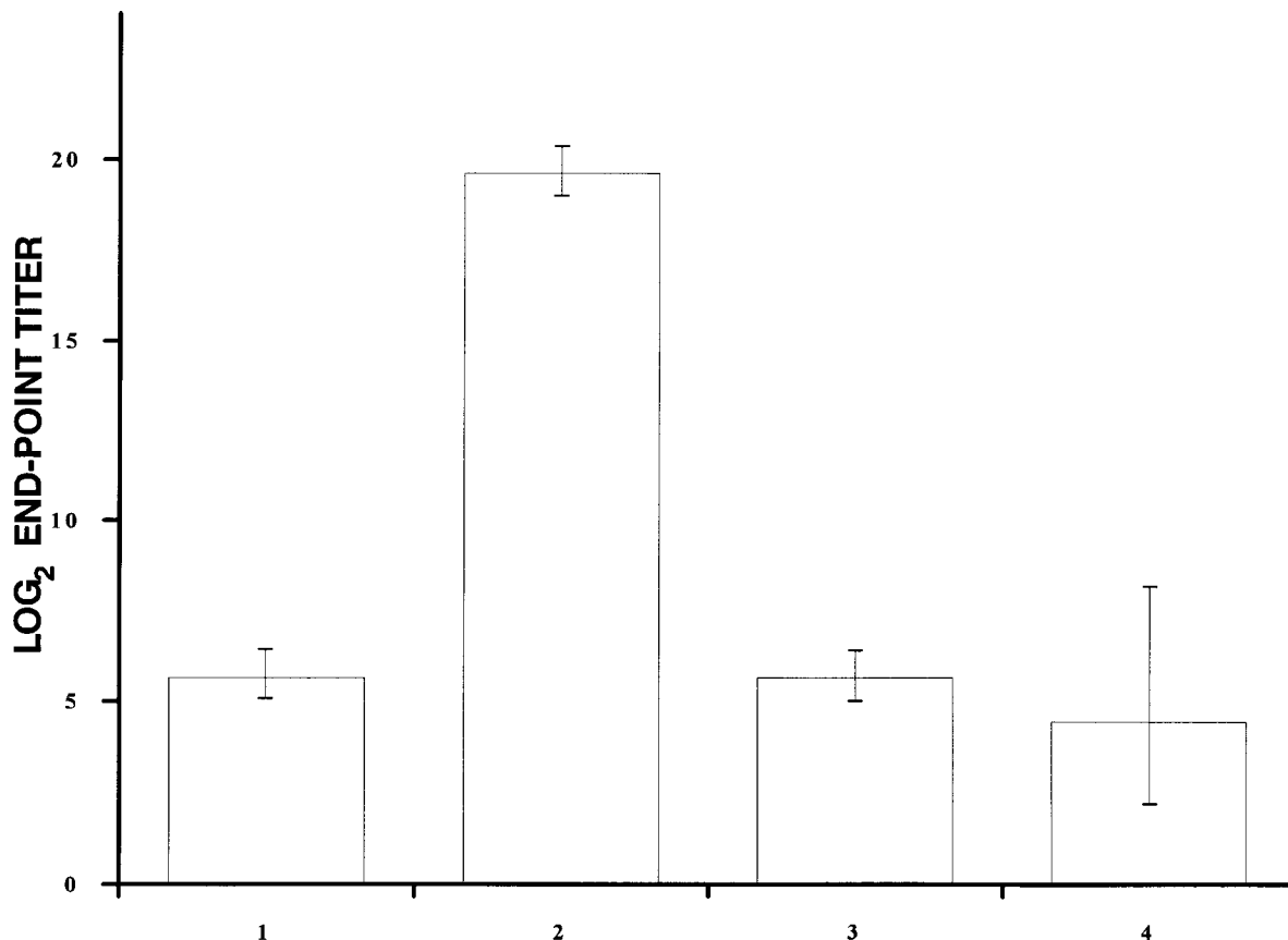
FIG. 3. CFA/I-specific serum IgG responses after oral immunization of mice. Shown are the geometric means \pm the standard errors of the CFA/I-specific serum IgG \log_2 endpoint titers that developed after oral immunization of mice with a 10^9 -CFU dose containing H683(pJRD184- asd + ) (1), H683(pJGX15C- asd + ) (2), \chi 6212(pJRD184- asd + ) (3), or \chi 6212(pJGX15C- asd + ) (4).
