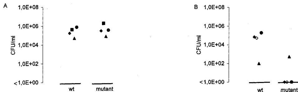
FIG. 5. Efficiency of colonization of wild-type and mutant bacteria on various organs of infected pigs. (A) Colonization of the wild-type strain 10 (wt) and the mutant strain 10 \Delta FBPS of the tonsils. Symbols: \blacklozenge , tonsil from pig 4664; \blacksquare , tonsil from pig 4665; \blacktriangle , tonsil from pig 4666; \bullet , tonsil from pig 4668. (B) Colonization of the specific organs. Symbols: \blacklozenge and \blacklozenge , pus from joints from pig 4664; \blacktriangle , pus from a joint from pig 4666; \bullet , CNS specimen from pig 4668. Each symbol represents the numbers of wild-type or mutant bacteria isolated from one particular organ, from one piglet.
