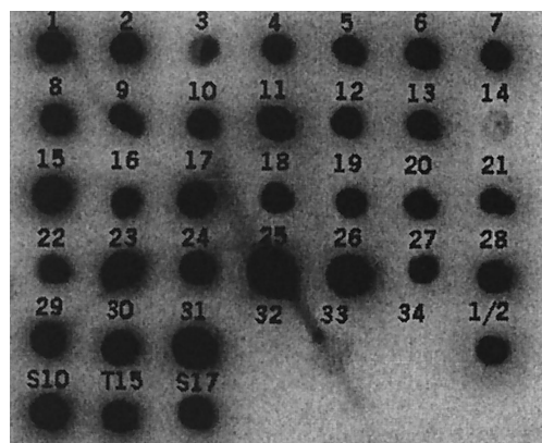
FIG. 4. Distribution of fbps among various S. suis serotypes. Chromosomal DNA (1 \mu g) was spotted onto nitrocellulose membrane and hybridized with a ^{32} P-labeled fbps probe. Serotypes were spotted as indicated. S10, S. suis serotype 2 MRP + EF + ; T15, S. suis serotype 2 MRP - EF - ; S17, S. suis serotype 2 MRP + EF* (23).
