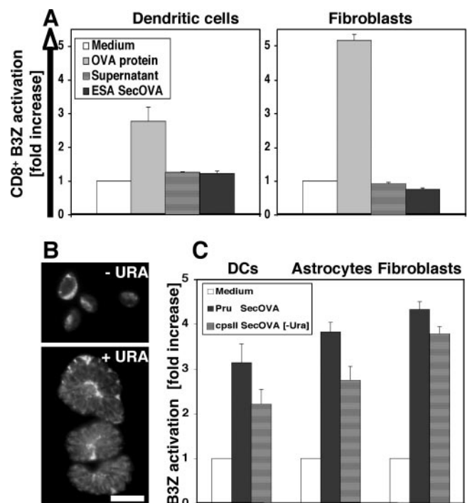
FIG. 3. MHC-I presentation of SecOVA from intracellular parasites versus lysed cell/parasite supernatant. (A) IFN- \gamma /TNF- \alpha -primed H-2K b BM-DCs and fibroblasts were incubated for 16 h with either OVA protein (500 \mu g/ml), concentrated supernatant from a lysed-out culture of \sim 5 \times 10^7 Prugniaud \Delta HXGPRT SecOVA parasites, or excreted/secreted antigens from 5 \times 10^4 Prugniaud \Delta HXGPRT SecOVA tachyzoites, and MHC-I/OVA presentation was measured using the B3Z cell assay; the number of parasites used corresponds to conditions employed in antigen presentation assays. B3Z cells were activated only when APCs were incubated with large amounts of exogenous soluble OVA (shown are averages for three experiments performed in triplicate \pm SD). (B) RH \Delta cpsII T. gondii parasites (15) engineered to secrete OVA into the PV were incubated with or without 0.2 mM uracil (URA) prior to staining with polyclonal anti-OVA. In these uracil auxotrophs, replication (and therefore cytolysis) is dependent on uracil, but parasites remain alive for several days, continuing to metabolize and secrete OVA protein into the PV. Bar = 10 \mu m. (C) IFN- \gamma /TNF- \alpha -primed H-2K b BM-DCs, astrocytes, and fibroblasts were incubated for 16 h with 5 \times 10^4 wild-type Prugniaud \Delta HXGPRT (Pru) SecOVA parasites or 5 \times 10^4 nonreplicating RH \Delta cpsII SecOVA parasites in the absence of uracil (-Ura). MHC-I presentation of SecOVA (detected using the B3Z cell assay) did not require parasite replication or host cell cytolysis, suggesting an endogenous origin of the presented antigen (average results from five or more experiments performed in triplicate \pm SD).
