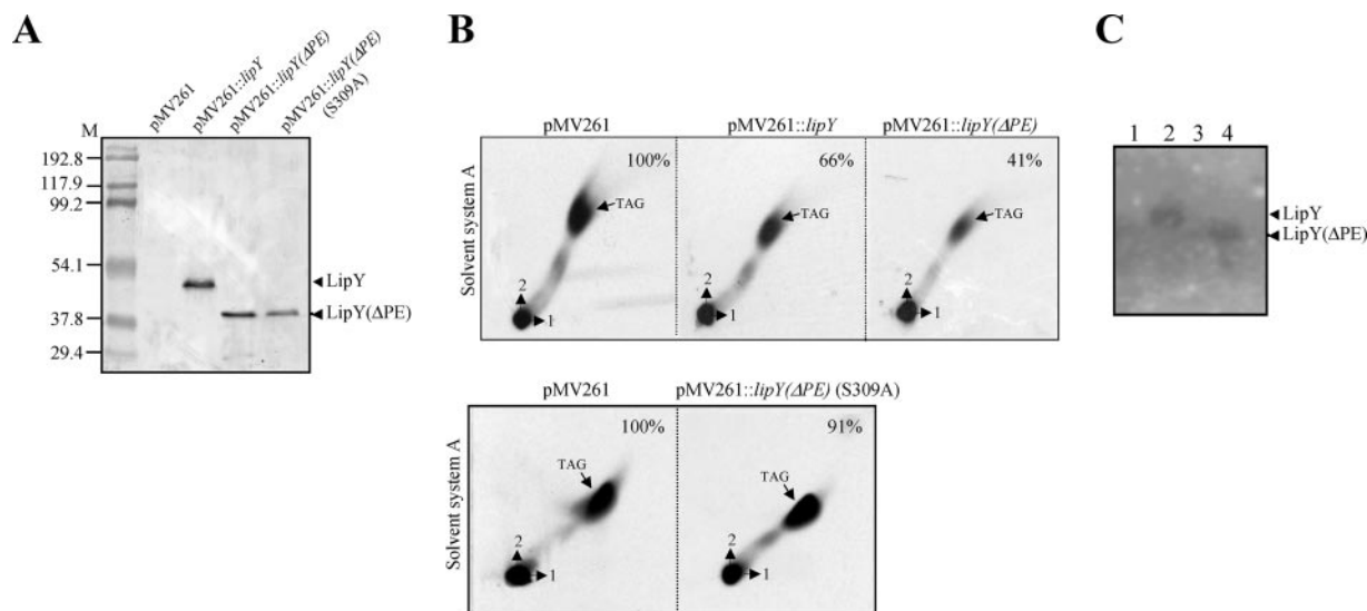
FIG. 4. Overexpression and lipolytic activity of LipY and LipY( \Delta PE) in M. bovis BCG. (A) lipY and lipY ( \Delta PE), as well as a version of lipY ( \Delta PE) carrying the S309A mutation [encoding LipY( \Delta PE)(S309A)], were cloned in pMV261, and the resulting plasmids were introduced into M. bovis BCG. The expression of the proteins in each lysate was assayed by Western blotting using rat anti-LipY( \Delta PE) antibodies. Equal protein amounts (20 \mu g) were separated on a 10% SDS-PAGE gel. (B) Recombinant M. bovis BCG cultures were labeled with 1 \mu Ci/ml [ ^{14} C]acetate for 24 h. Apolar lipids were extracted and equal counts were applied onto silica gel plates. Separation was done using solvent system A and plates were exposed overnight to film. The percentage of TAGs present in each strain (with regard to the reference strain presence, which was arbitrarily set to 100%) was determined by densitometry and is indicated in the upper right corner of each TLC plate. (C) Gel overlay assay. M. bovis BCG lysates were separated by SDS-PAGE. Following renaturation, the gel was laid on top of an agar plate containing tributyrin as a substrate. A clear halo forms when the overexpressed lipase is active. Lanes: 1, M. bovis BCG pMV261; 2, M. bovis BCG pMV261:: lipY ; 3, M. bovis BCG pMV261:: lipY ( \Delta PE)(S309A); 4, M. bovis BCG pMV261:: lipY ( \Delta PE).
