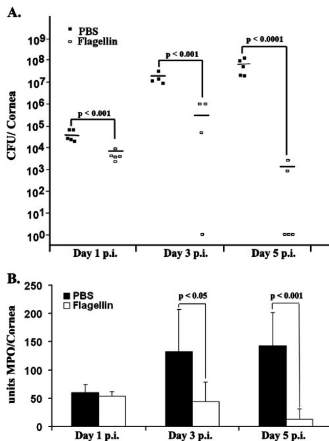
FIG. 3. PMN infiltration and bacterial clearance in flagellin-pretreated corneas. Mice were treated with PBS ( n = 5 ) or flagellin ( n = 5 ) as described in the text, followed by ocular inoculation of 1 \times 10^6 CFU of P. aeruginosa strain ATCC 19660 per cornea as described in the legend to Fig. 2. At the indicated times after infection, the corneas were excised and subjected to plate bacterial counting (A) or determination of MPO activity as a parameter for PMN infiltration (B). In panel B the bars indicate the arithmetic mean and the error bars indicate the standard error of the mean for five mice in each group. P values were generated using paired Student's t test for the MPO assay and the Mann-Whitney test for bacterial counts.
